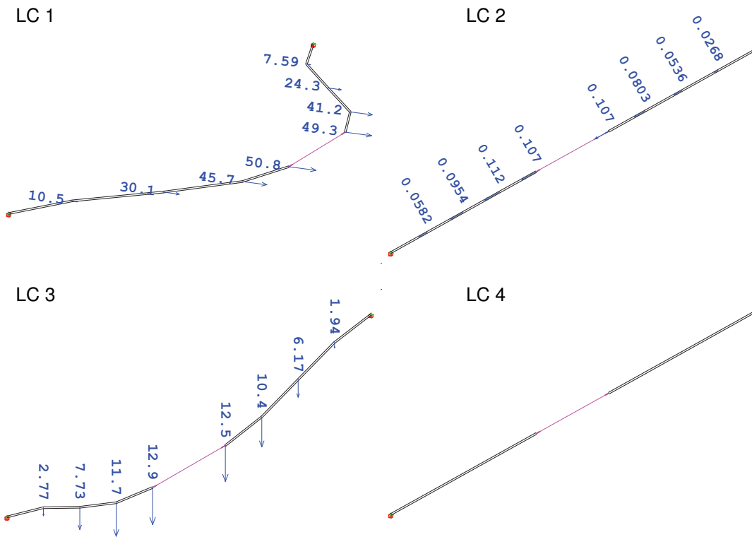
Figure 2: Displacement Results for KF coupling for LC 1-4
